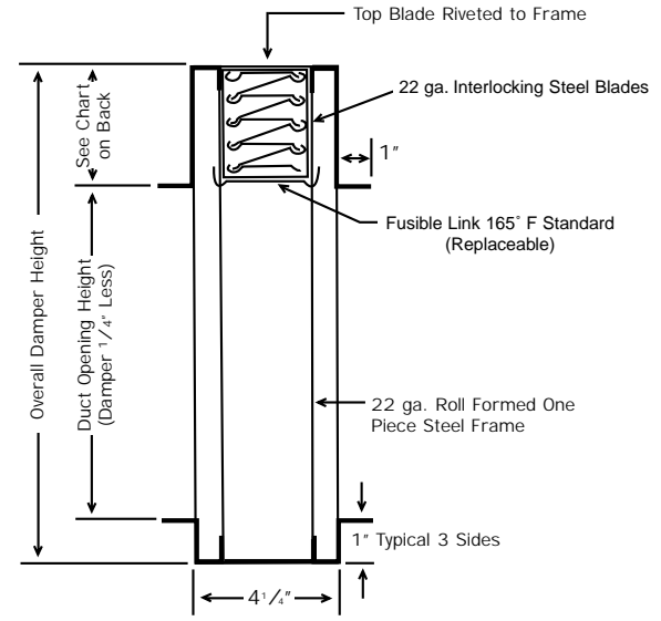
VERTICAL MOUNT MODEL 5530
